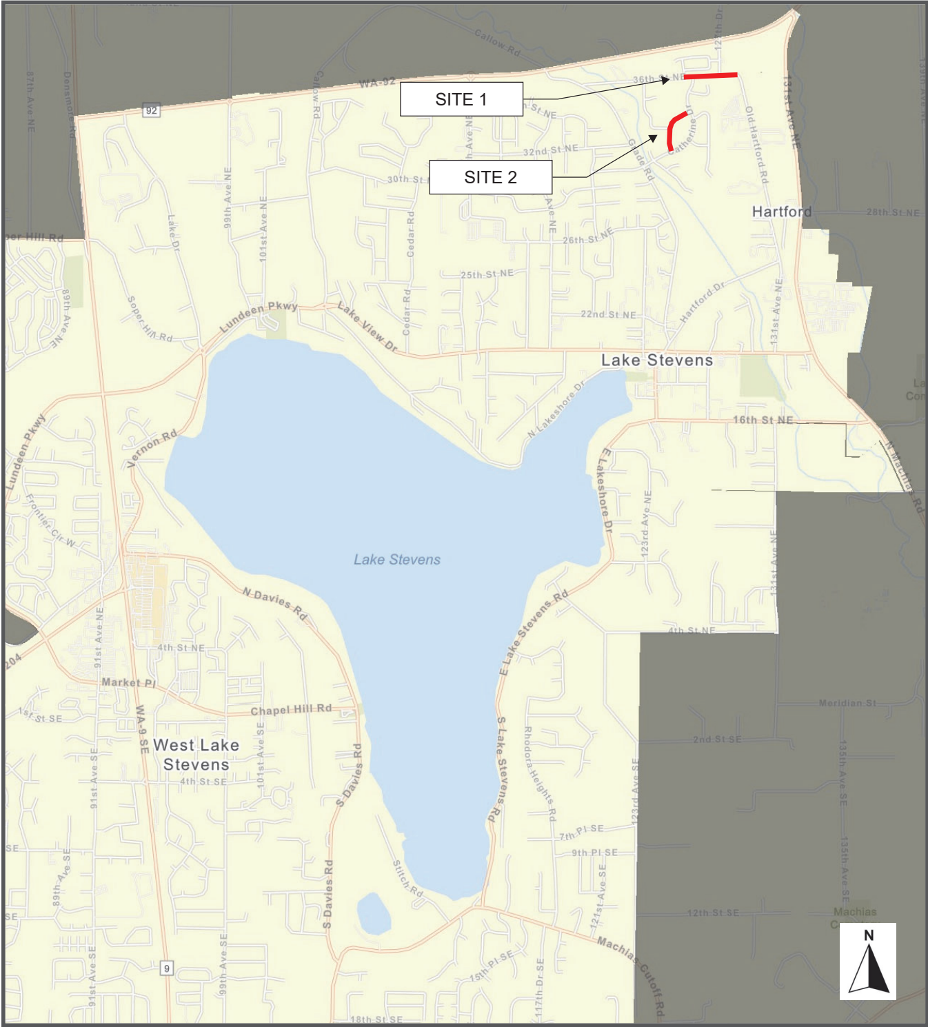
VICINITY MAP
