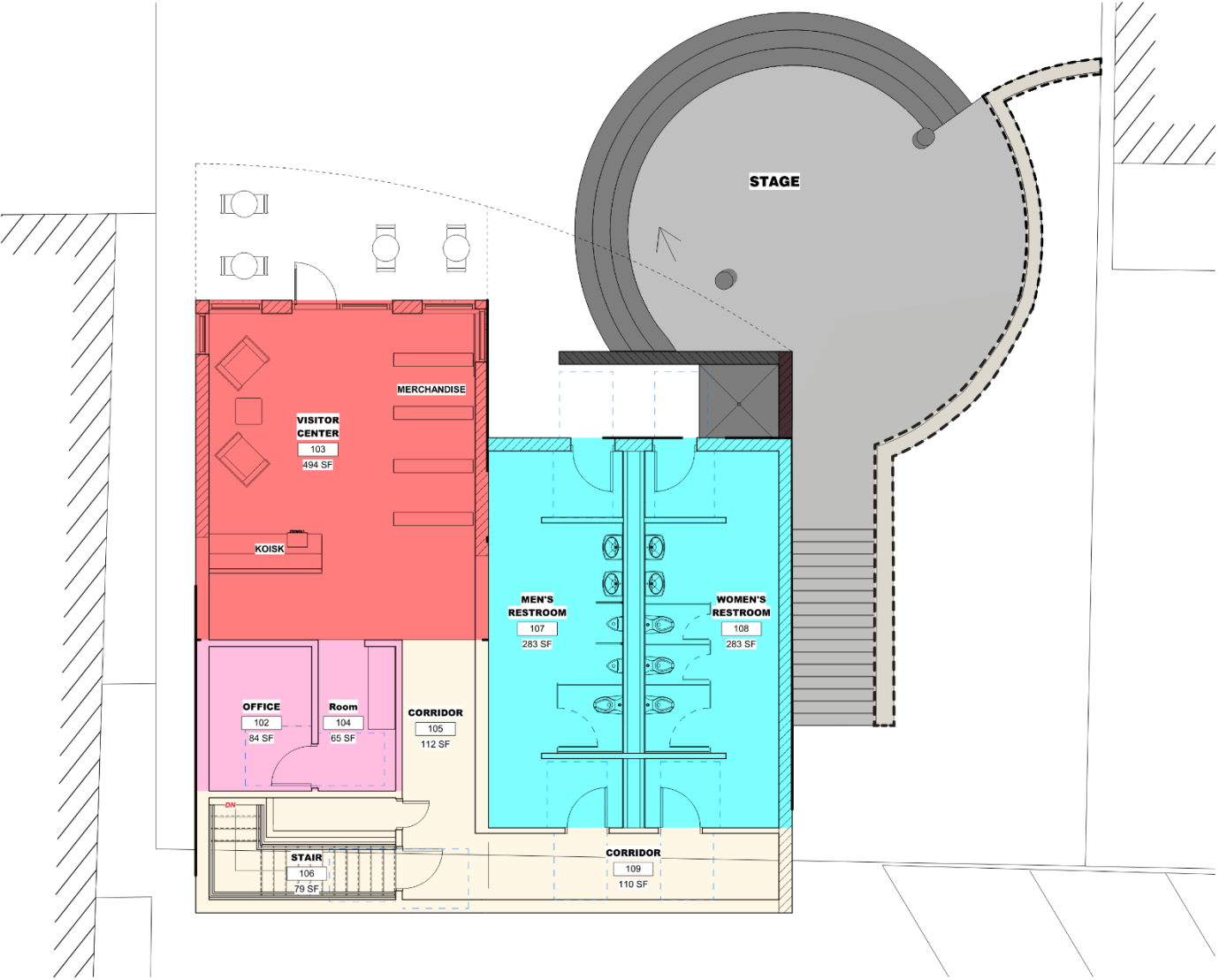
1 PROPOSED FLOOR PLAN A.1 1/4" = 1'-0"
