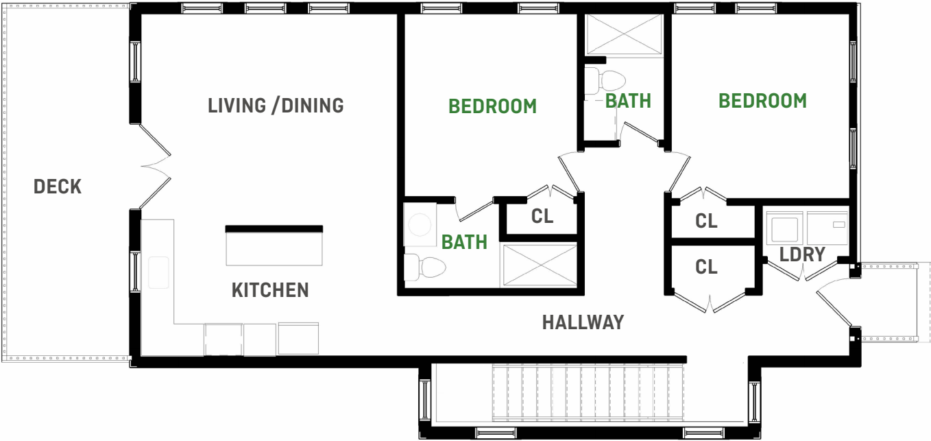
FIRST FLOOR
