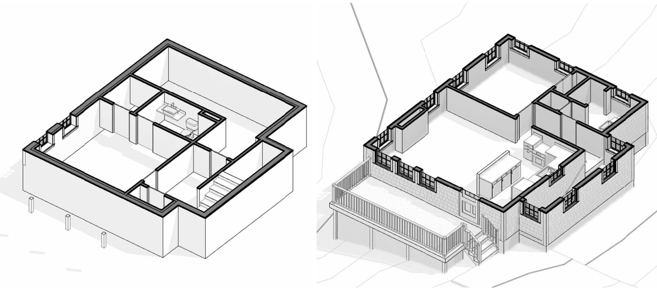
3D FLOOR PLAN - BASEMENT
