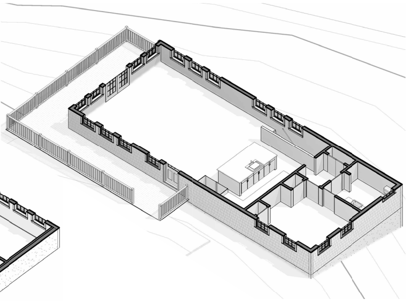
3D FLOOR PLAN - FIRST FLOOR
