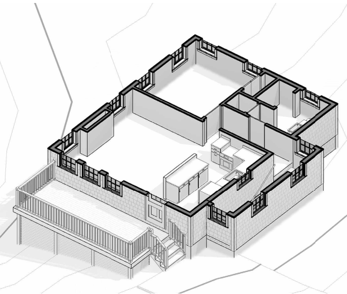
3D FLOOR PLAN - FIRST FLOOR
